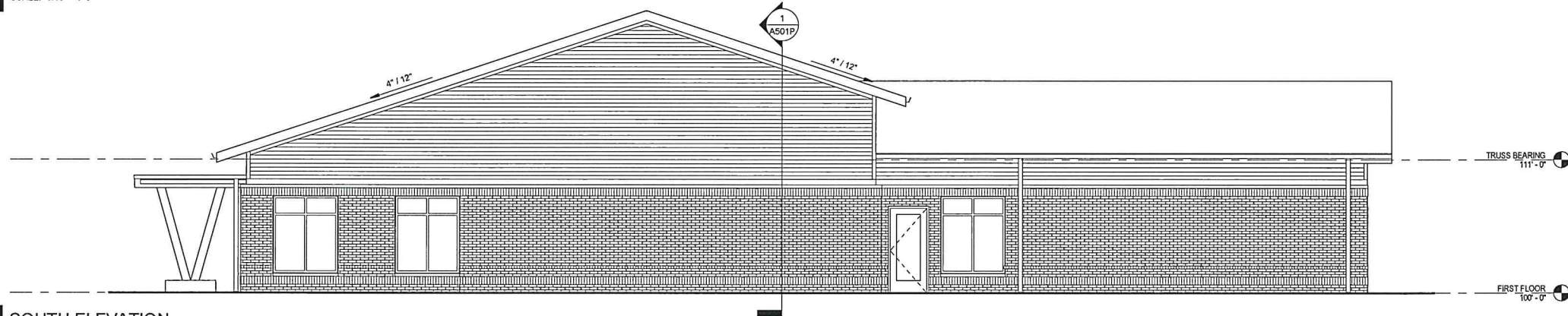
2 SOUTH ELEVATION
