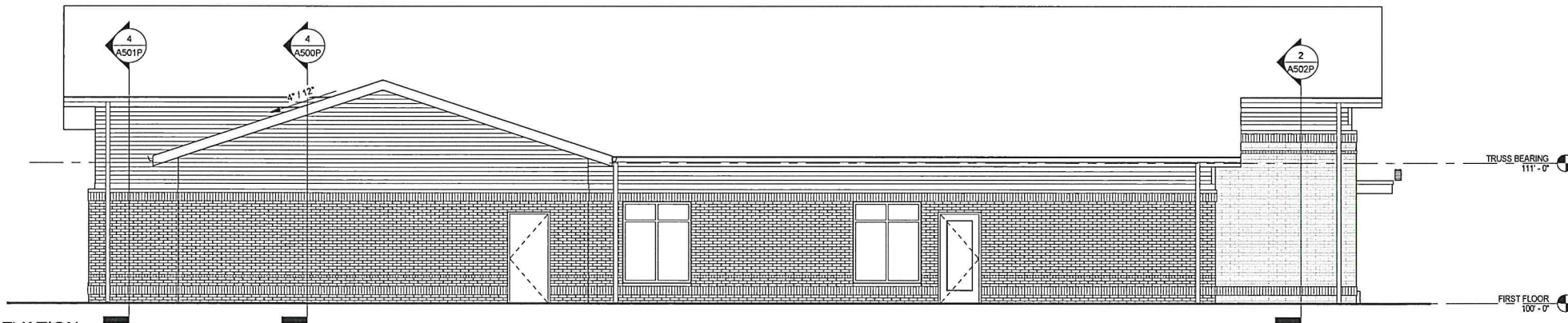
3 EAST ELEVATION
